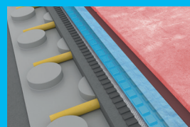
HEATING DISTRIBUTION
