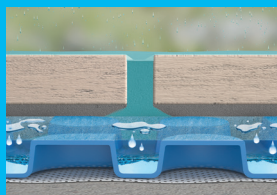
WATERPROOFING
